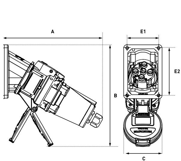
PLUG ON 30° INCLINED SOCKET-OUTLET
